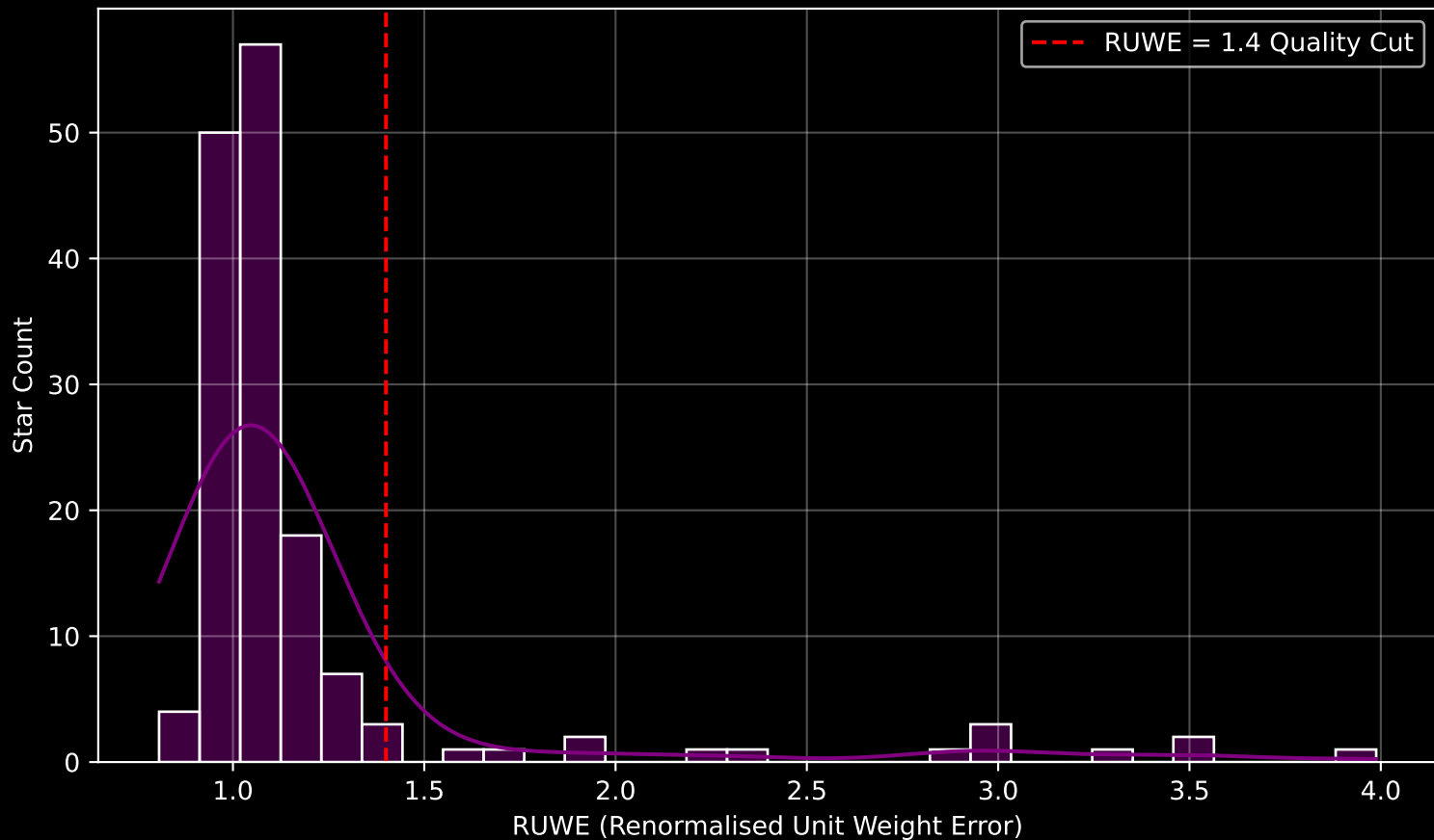
GAPOGEE DR17 Field [120+18] RUWE Distribution (n= 153)
